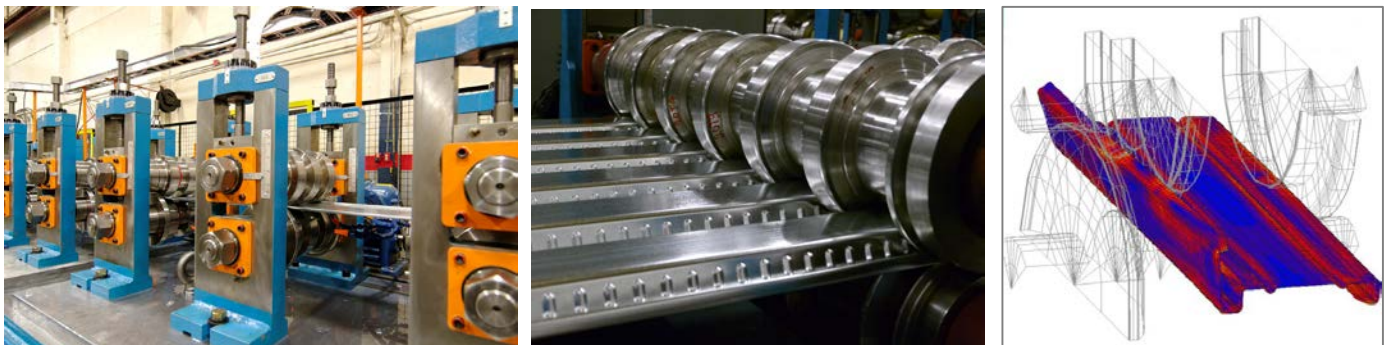
Figure 2: Roll Forming Process
